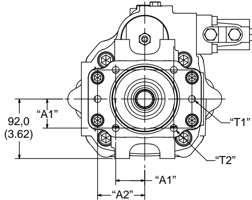
Right hand rotation with Load Sensing Control
