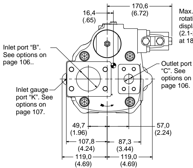
Right hand rotation with Load Sensing Control
