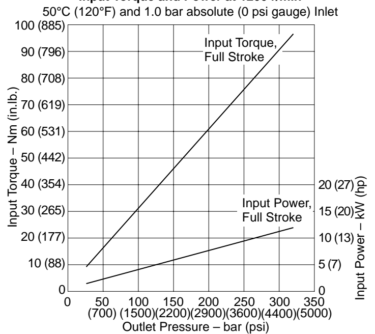
Input Torque and Power at 1200 r/min
