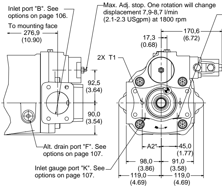
Right hand rotation with 2-bolt "A" flange and Load Sensing Control
